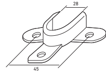
SopORTE para rodamiento Ø28 mm Ball bearing support Ø28 mm Support pour roulement Ø28 mm Supporto per cuscinetto Ø28 mm
