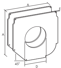
Placas contención 300/45 Safety plates 300/45 Plaques 300/45 Piastra di contenimento 300/45
