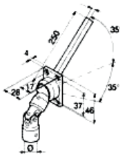
Snodo 35° placa 4 Taladros Joint 35° with 4 holes plate Cardán 35° avec plaque 4 trous Snodo 35° con placca 4 fori
